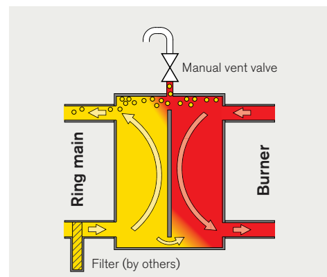
Separation into different temperature zones saves energy and reduces costs
